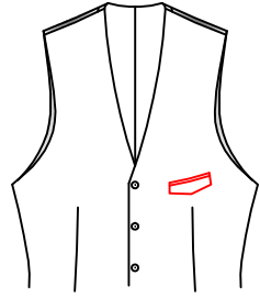
V-4135 Left slant double besom chest pocket with diamond flap
