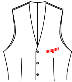
V-4138 Left slant double besom chest pocket with loop and button
