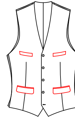
V-41A7 Double besom lower pocket with flap+welt breast pockets
