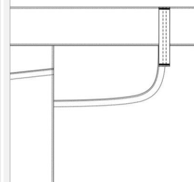
N102 jean pocket without watch pocket
